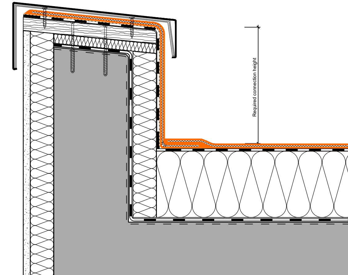
Scale 1:5 (Waterproofing layers are elevated)
